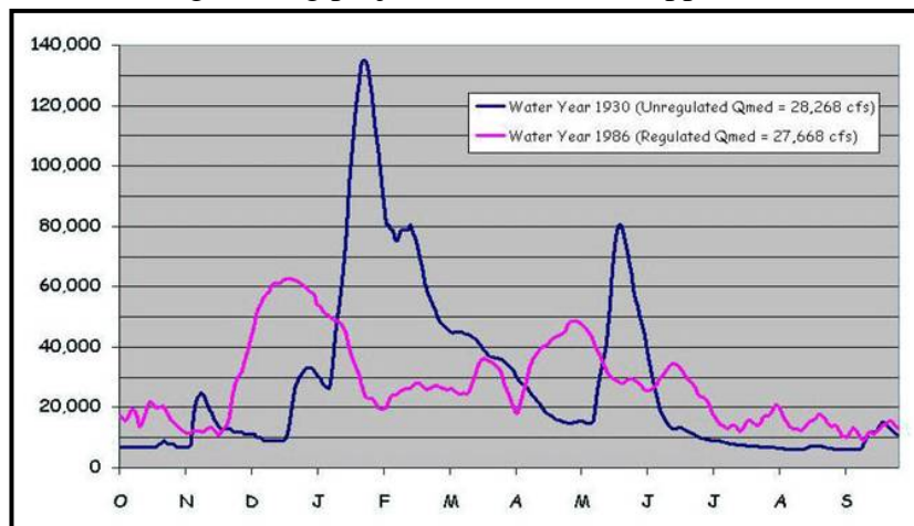
Figure 4. Hydrograph of the White River at Clarendon, Arkansas, Showing Flow Alteration Following Construction and Operation of Dams on the Upper White River and Tributaries
